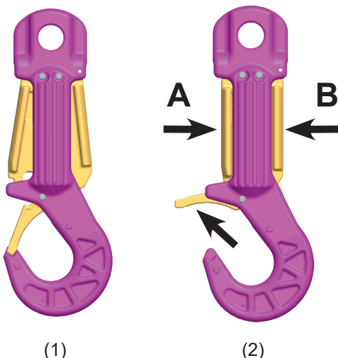
Pic. 6: The ROV-HOOK opening mechanism
