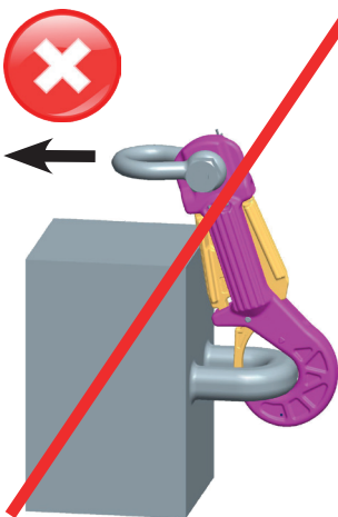
Pic. 12: ROV-HOOK loaded in the direction of the hook tip
