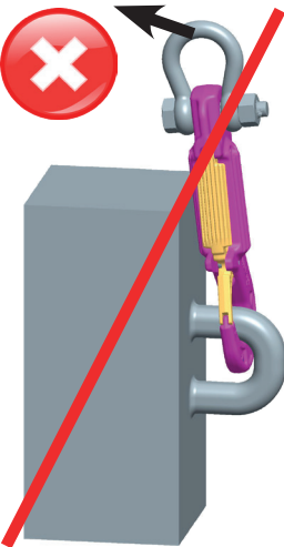
Pic. 11: ROV-HOOK with load at the side
